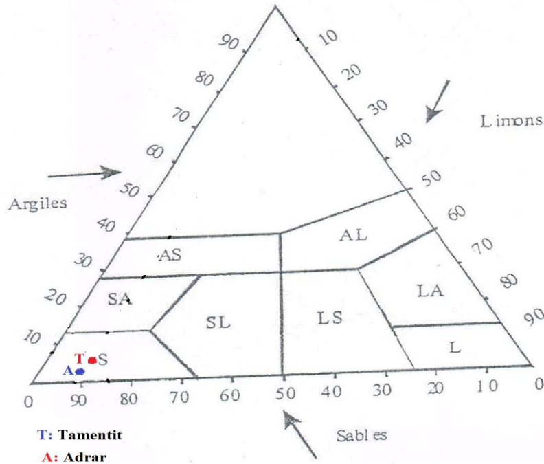
Figure n°19: Triangle textural
