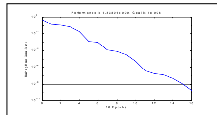
Fig.3.RMS error of the first classifier during the training process.
