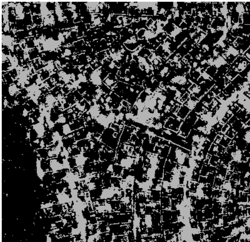
Figure III.22 : Image 3 (RVI).
