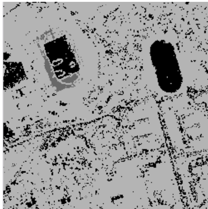
Figure III.26 : Image 4 (RVI).
