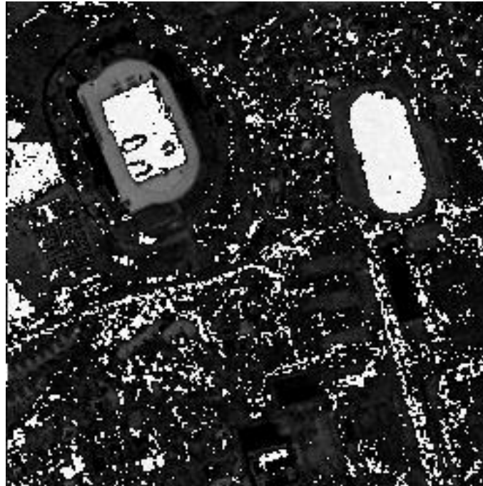
Figure III.25 : Image 4 (DVI).
