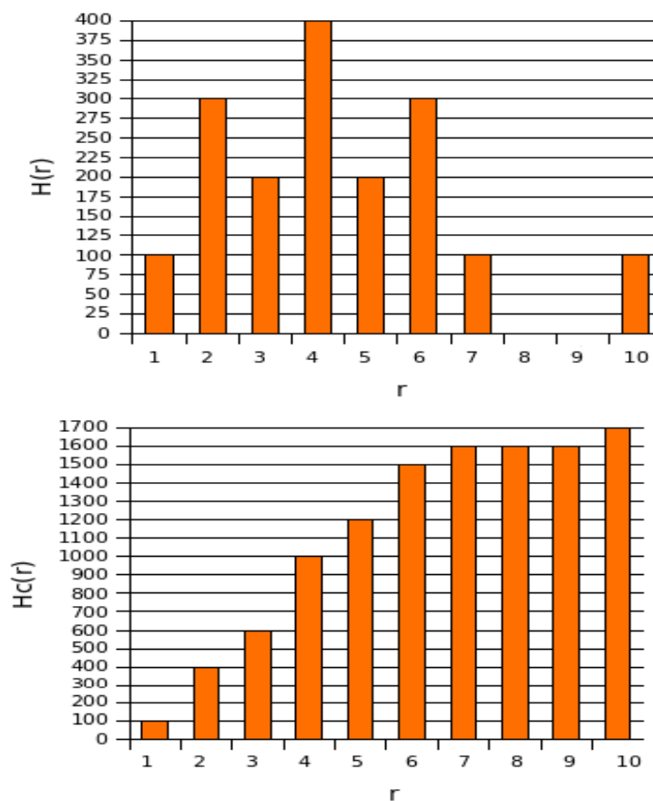
Figure I.5 :HISTOGRAMME
