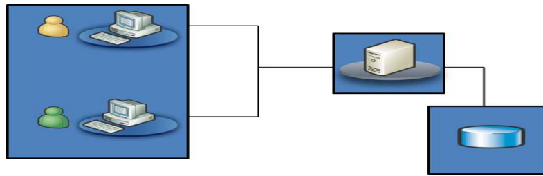
Figure I.5 : architecture 3-tiers
