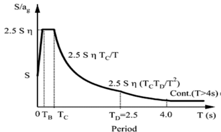
Figure III.5: Spectre de conception
