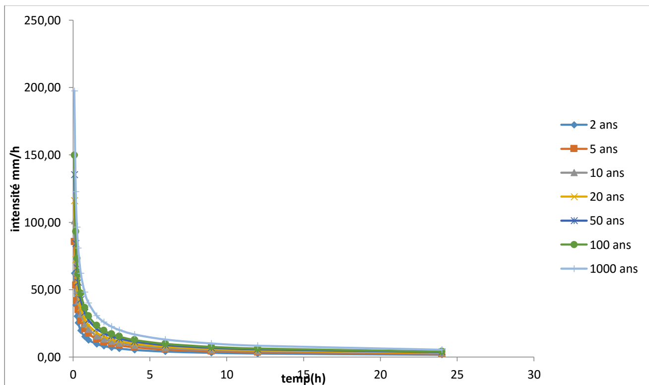
Figure IV.6 : Courbes IDF.
