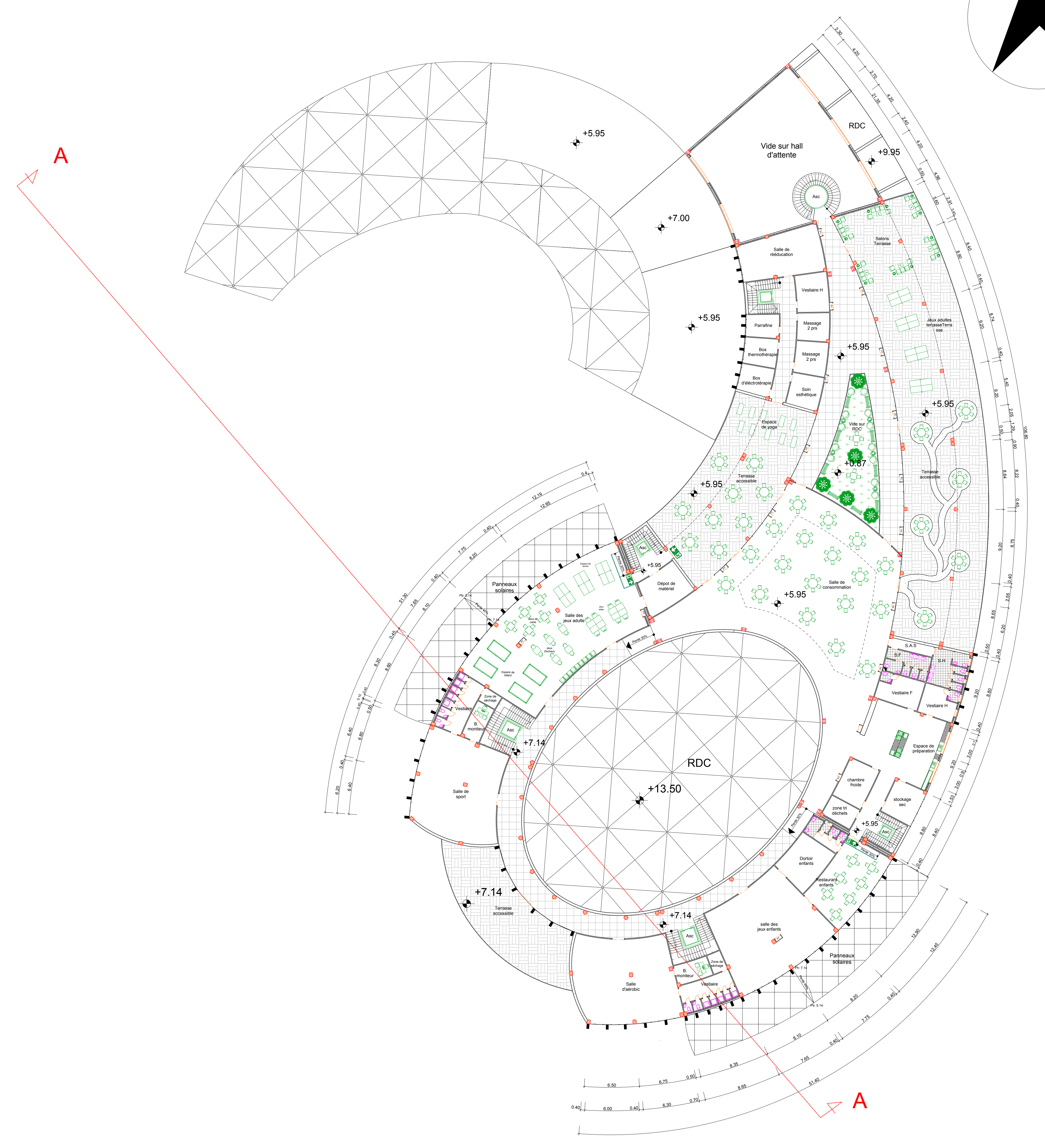
Plan R+1 (ech 1/200)
