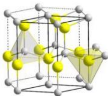
Figure 1.12 Structure Wurtzite [7].
