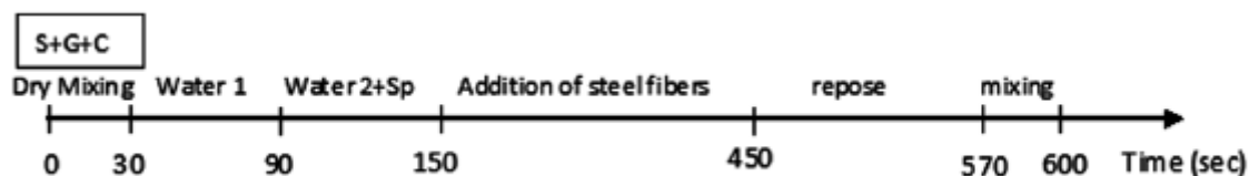
Figure II.2: Mixing procedure for FRSCC
