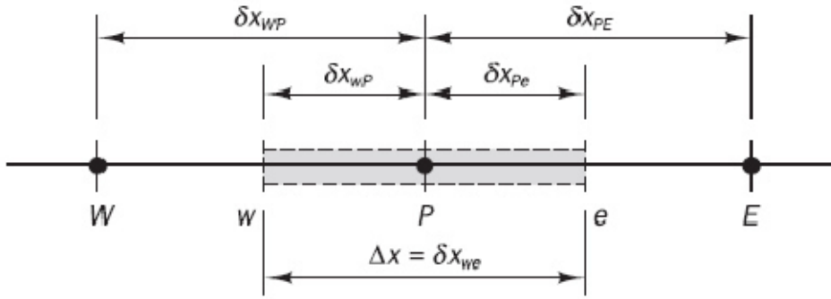
Figure II.5: Grid cells
