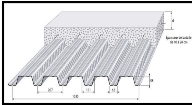
Figure 144. planchers collaborant
