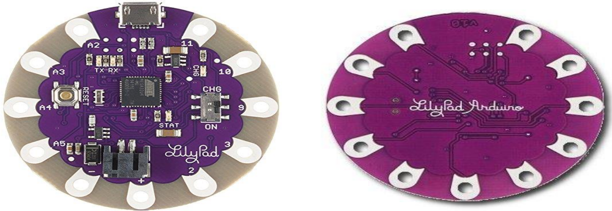
Fig.9: Arduino LilyPad
