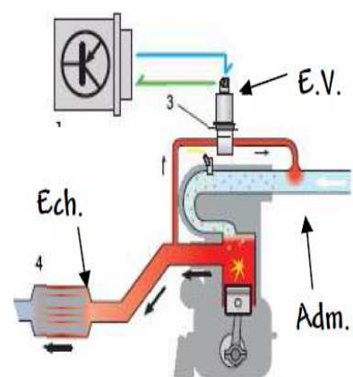
Figure I.16 principe de la recirculation
