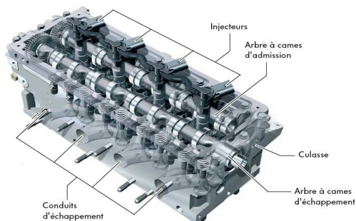
Figure I.4 La culasse
