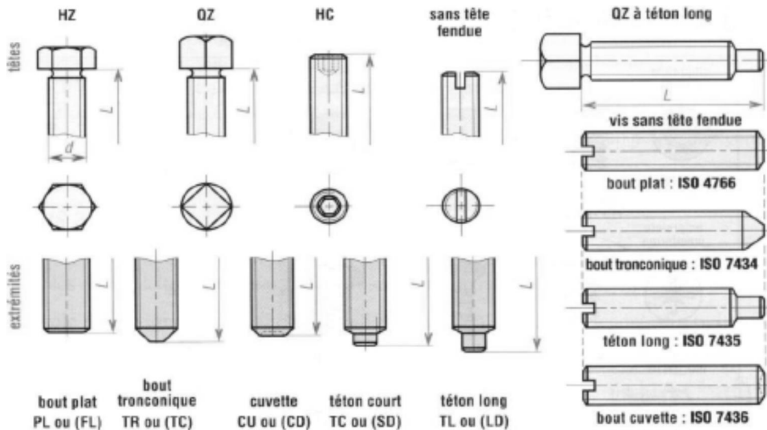
Figure II.3 : Vis de pression
