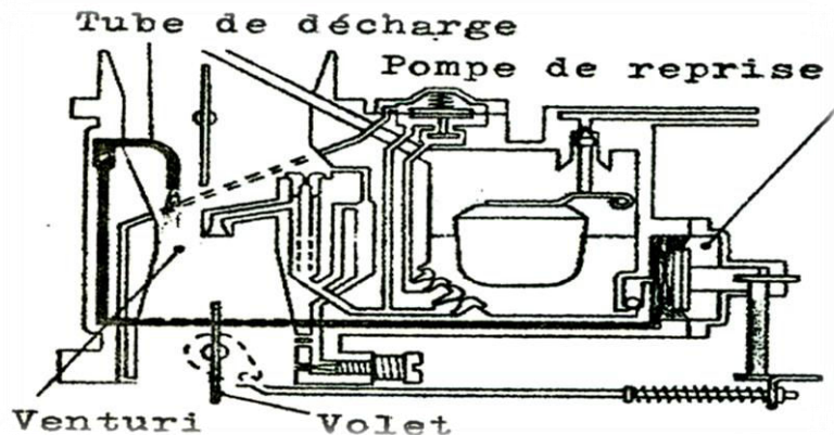
Figure II.35 : Circuit de reprise
