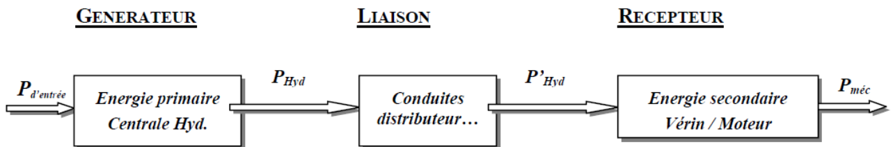
Figure 2.19. Constitution du circuit hydraulique
