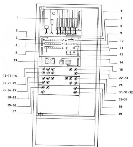
Figure 8. Tableau PLC -ELBO
