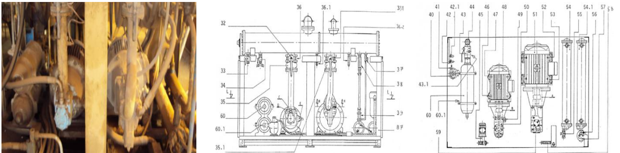
Figure 2.20. Centrale hydraulique
