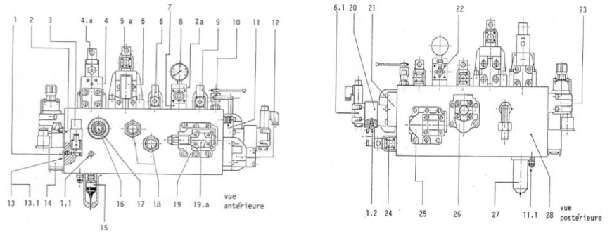
Figure 2.17. Bloc A2
