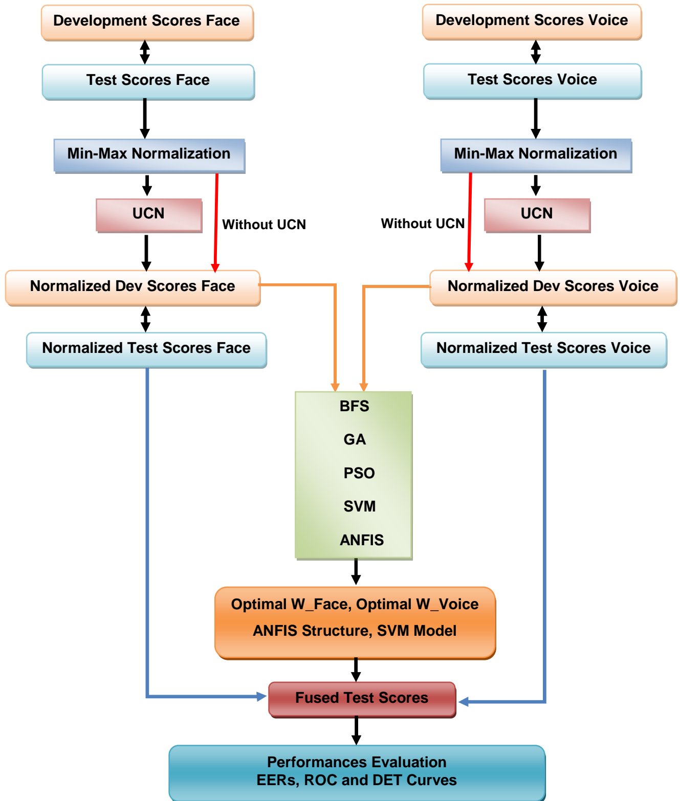
Figure 4.2: Multimodal biometric score-level fusion flowchart.
