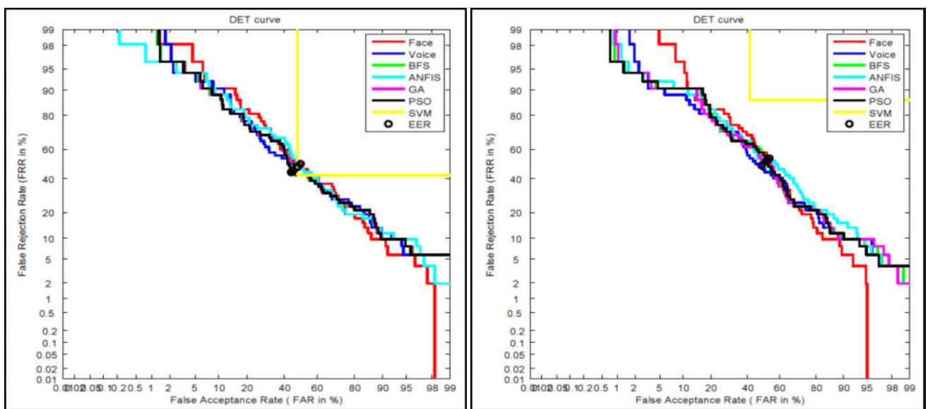
Figure 4.7: (a) DET curves for different fusion techniques under degraded data quality condition without UCN. (b) DET curves for different fusion techniques under degraded data quality condition with UCN.
