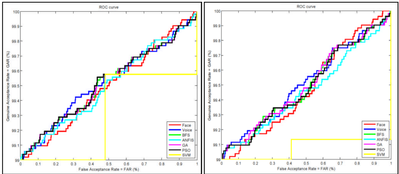
Figure 4.8: (a) ROC curves for different fusion techniques under degraded data quality condition without UCN. (b) ROC curves for different fusion techniques under degraded data quality condition with UCN.
