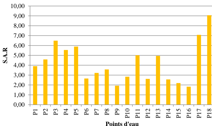
Figure III.16 : Variation du Sodium Absorption Ratio
