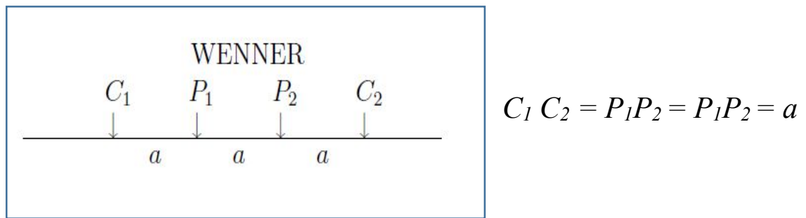
Figure 12: Technique WENNER
