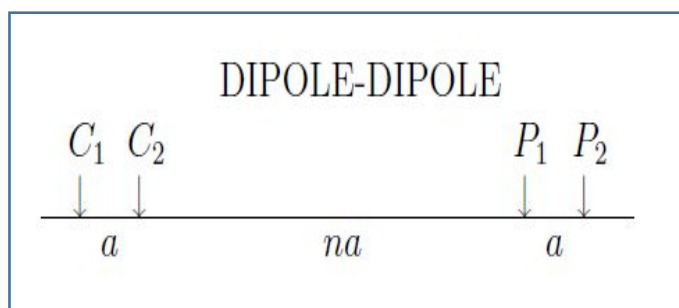
Figure 8: Technique Dipôle-dipôle
