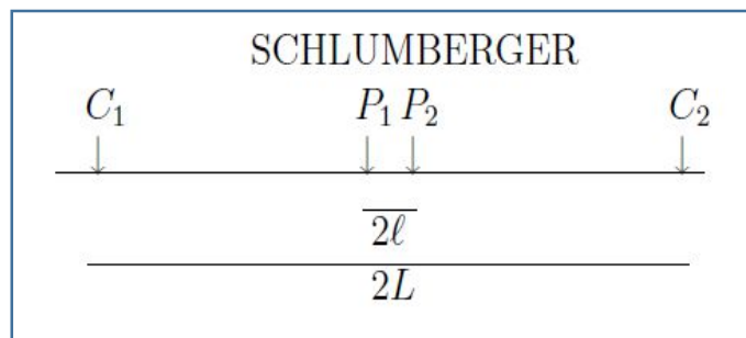
Figure 7: Technique Schlumberger
