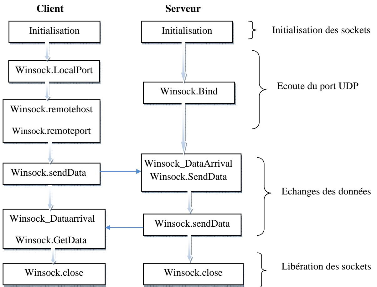
Fig.IV.3 Architecture client/ server TCP/IP
