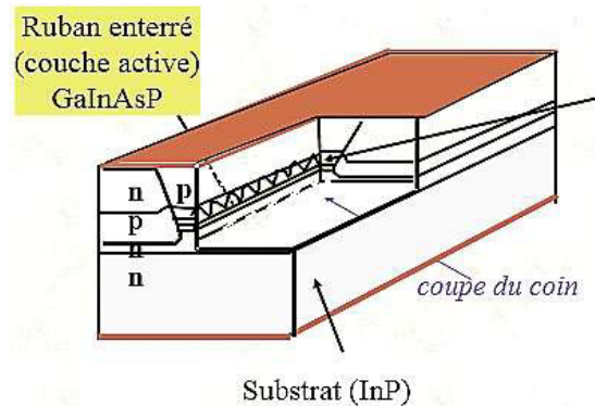
Figure 1.12 : Diode Laser
