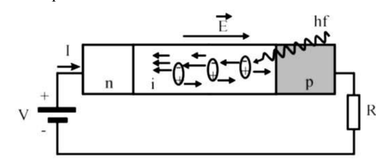
Figure 1.16:Photodiode a avalanche
