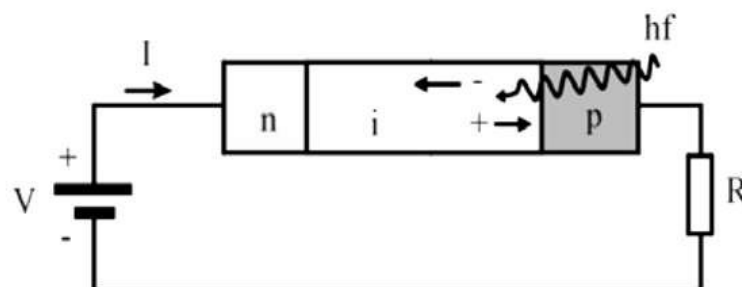
Figure 1.15 : Photodiode PIN
