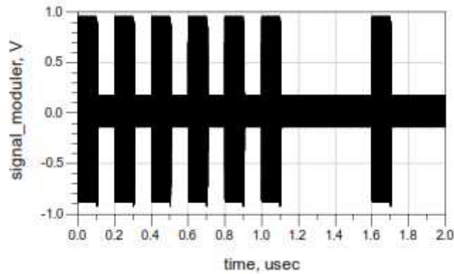
Figure 4.22: Signal modulé en amplitude.
