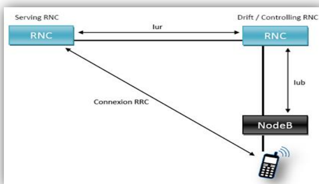
Figure II. 8: Serving RNC et Drift RNC dans UTRAN
