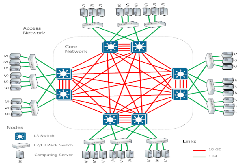
Figure II.4 : Architecture Two-tier [41].
