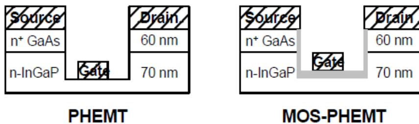
Figure I.7: Structures PHEMT et MOS-PHEMT
