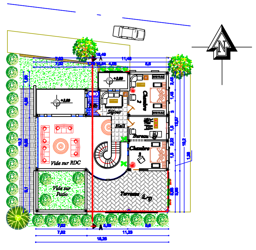
Plan R+1
