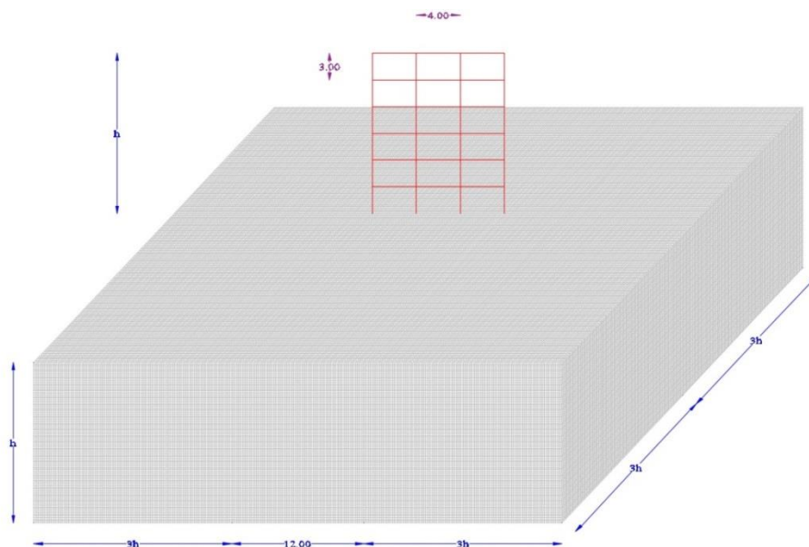
Figure 4.1 : structure (R+5).
