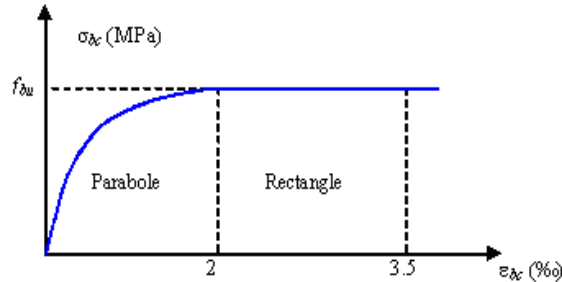
Figure I.4: Diagramme parabolite rectangle
